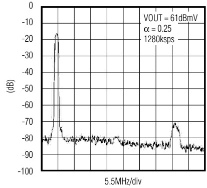
OUTPUT SPECTRUM
