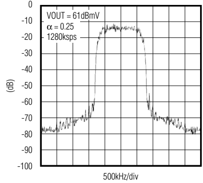
OUTPUT SPECTRUM
